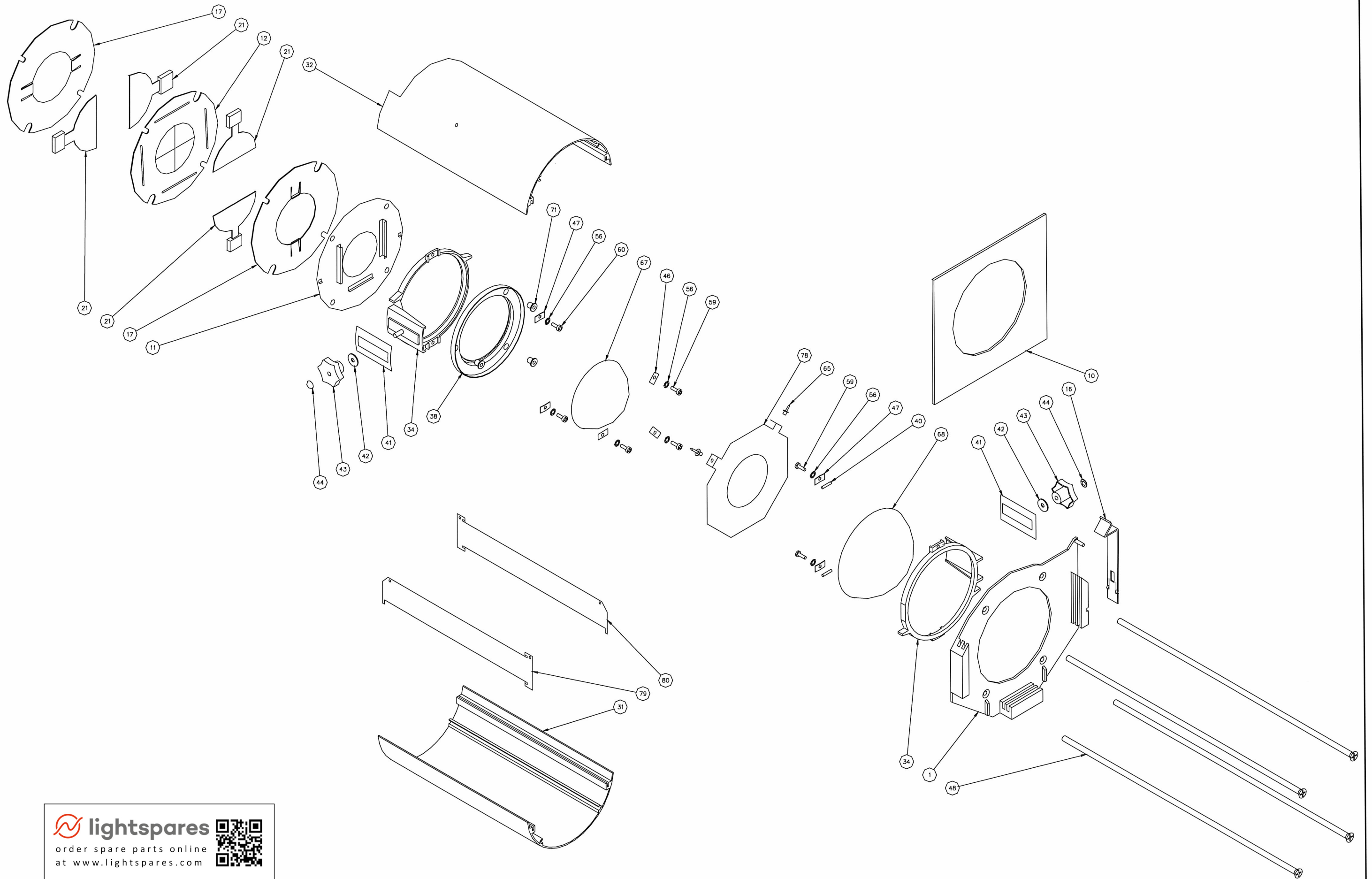
QUARTET 15/25 MK2 LENS ASSEMBLY
